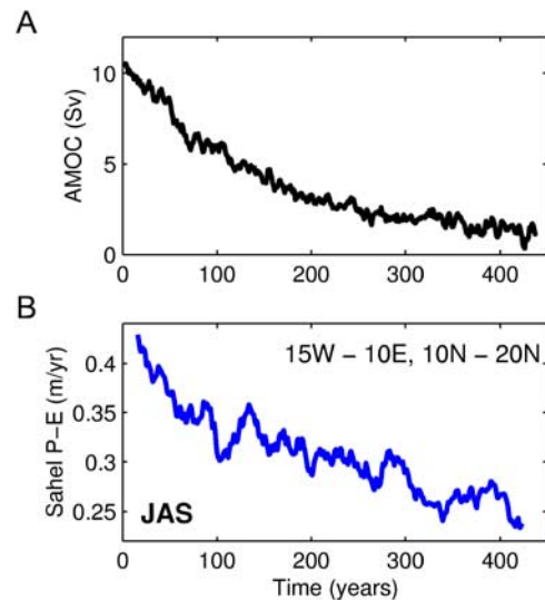
Figure 7. Results from the coupled general circulation models (CGCM) water-hosing simulation where the high northern seas are perturbed by a continuous freshwater input of 0.1 \text{ Sv} . (a) Temporal evolution of the Atlantic meridional overturning circulation (AMOC), starting from the equilibrium climate of the control run. Shown is the maximum of the overturning stream function north of 40^\circ\text{N} smoothed with a 5-year boxcar average. (b) Summer, i.e., July/August/September (JAS), net precipitation (total precipitation minus evapotranspiration) averaged over the West African Sahel ( 15^\circ\text{W}\text{--}10^\circ\text{E} , 10^\circ\text{N}\text{--}20^\circ\text{N} ) smoothed with a 30-year boxcar average.
