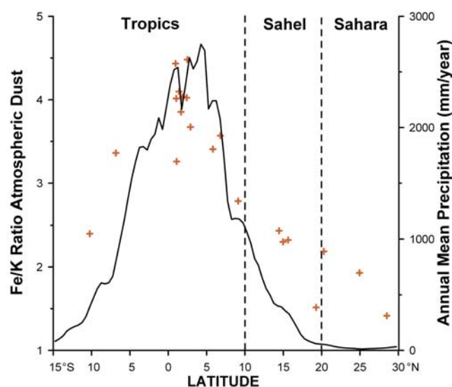
Figure 2. Comparison of Fe/K of atmospheric dust sampled in the period from February–March 1998 on R/V Meteor along western Africa (data from Stuut et al. [2005]) and annual mean precipitation at 18°W (Global air temperature and precipitation are available at http://climate.geog.udel.edu/~climate/html_pages/archive.html ).
